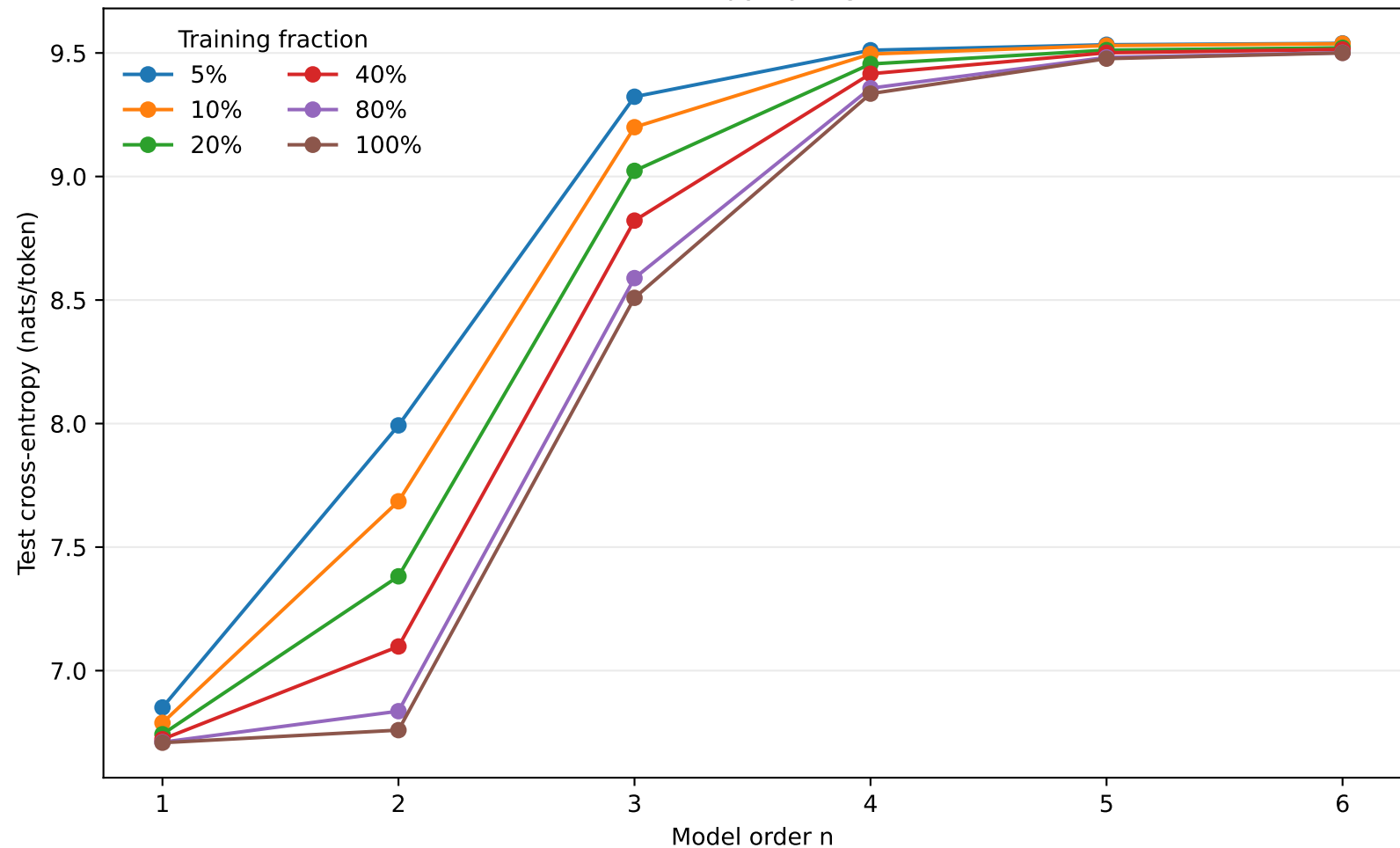
Test cross-entropy by n-gram order
