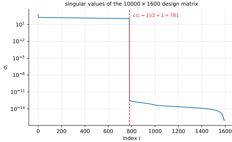
Fig. 3.5 Singular values of the 10000 \times 1600 Ising design matrix (3.94) for L = 40 . The spectrum collapses precisely at the index L(L-1)/2 + 1 = 781 predicted by Proposition 3.14: the rank deficiency is a property of the features, not of the sample.
