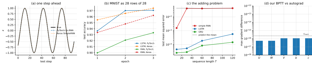
Fig. 11.5 (a) One-step-ahead forecasts of the sine wave of Section 11.8.1 on the held-out segment, from nn.RNN and from SimpleRNN ; both lie on the true curve at a root-mean-square error of 0.003. (b) Test accuracy against epoch for MNIST read row by row, Table 11.1. (c) The adding problem: mean squared error against sequence length for the three cells, with the error of predicting the mean shown dotted. The simple RNN leaves the dotted line only at T = 10 . (d) The largest disagreement between our BPTT recursion, Eqs. (11.15)–(11.18), and the same gradients from automatic differentiation, against the double-precision unit roundoff.
