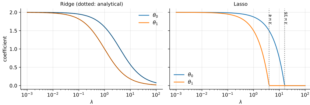
Fig. 3.2 Coefficient paths for the toy problem (3.70). The Ridge coefficients (left) follow the analytical result (3.73), shown dotted, and approach zero only asymptotically. The Lasso coefficients (right) reach zero at the finite thresholds \lambda = 4 and \lambda = 16 predicted by Eq. (3.63).
