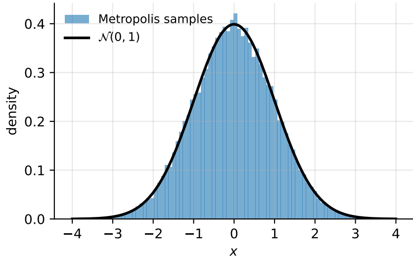
acceptance 0.50, \tau = 4.3
