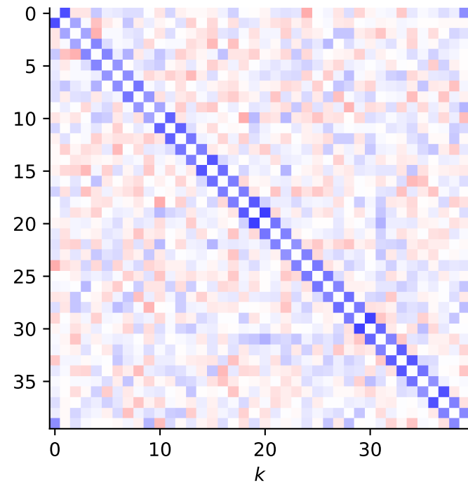
Ridge, \lambda = 0.01
