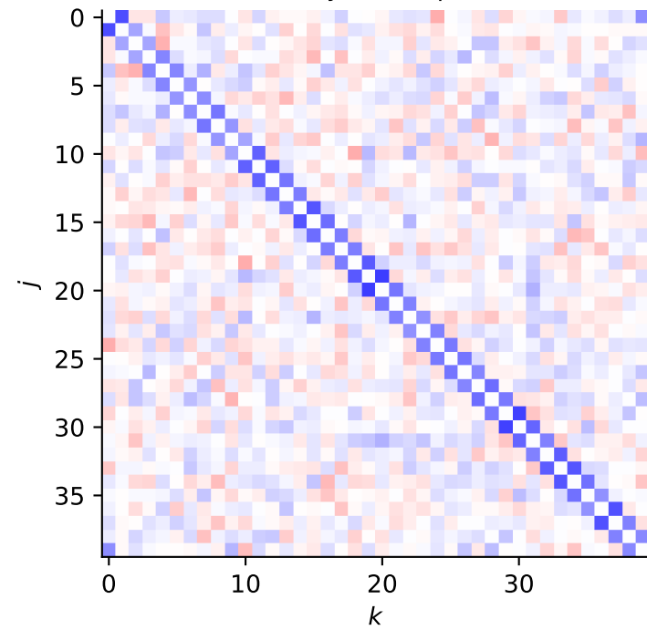
ordinary least squares
