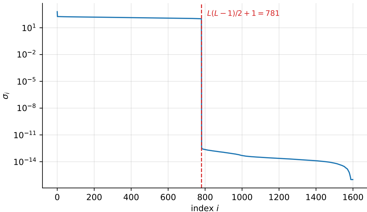
singular values of the 10000 \times 1600 design matrix
