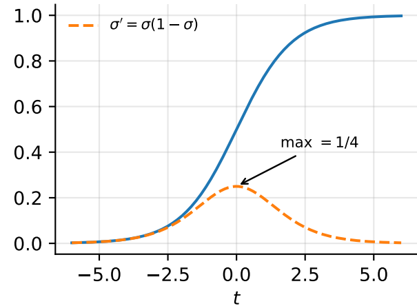
sigmoid \sigma(t)
