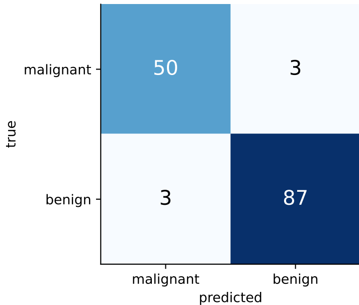
confusion matrix
