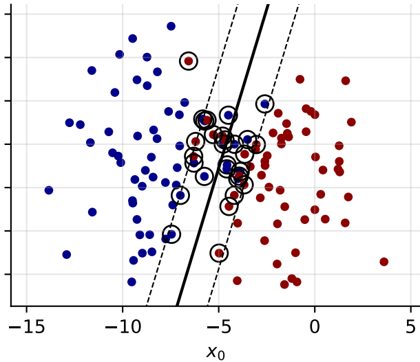
C = 10 : 29 SV, margin 3.01
