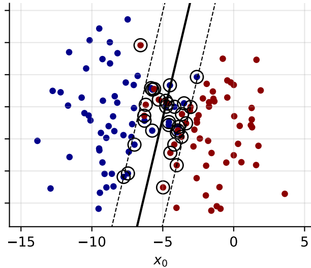
C = 0.1 : 32 SV, margin 3.43
