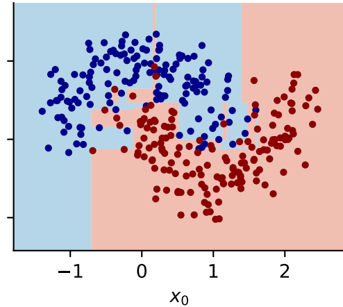
depth \infty train 1.000 / test 0.900
