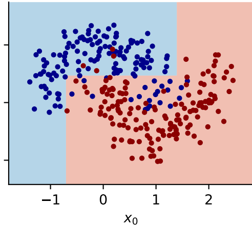
depth 3 train 0.910 / test 0.810
