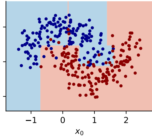
depth 5 train 0.947 / test 0.890
