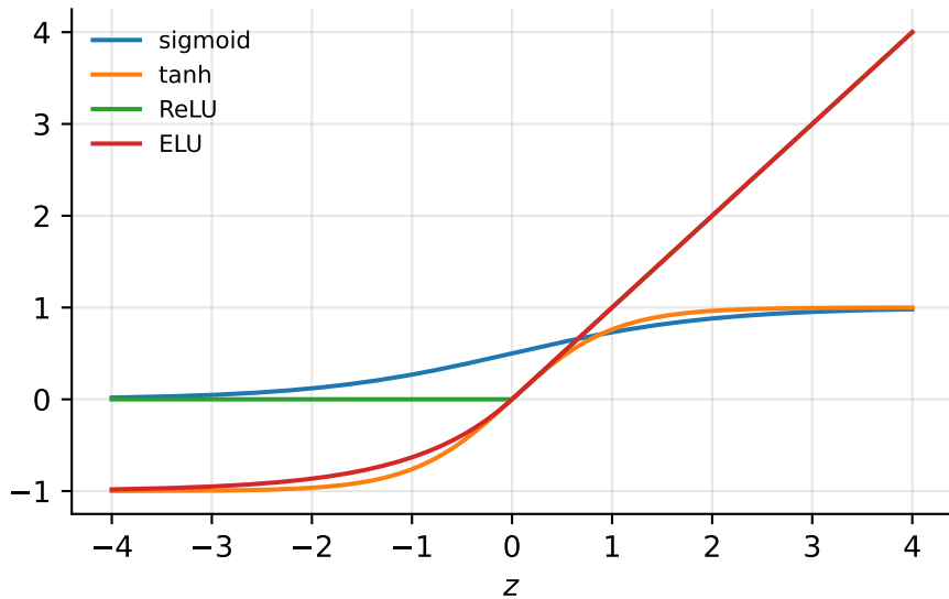
activation f(z)
