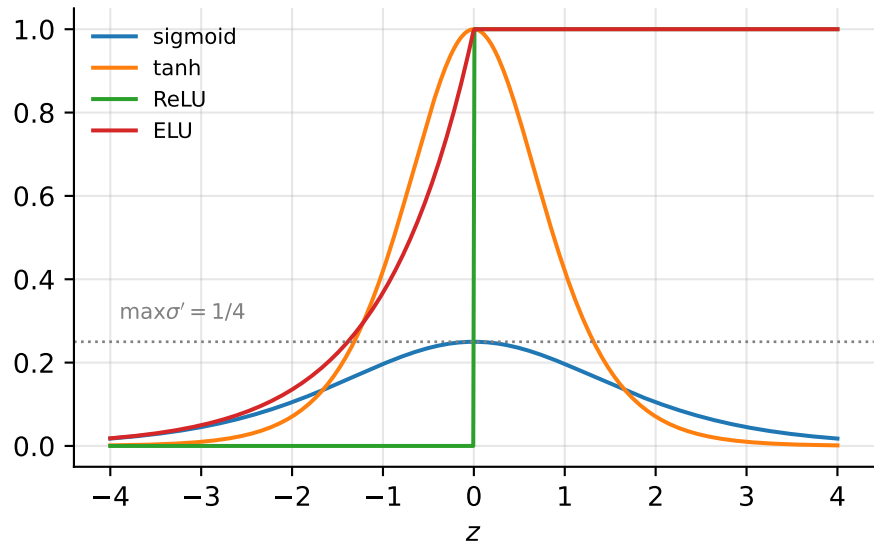
derivative f'(z)
