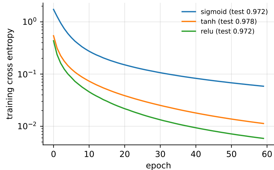
64-50-10 on the digits
