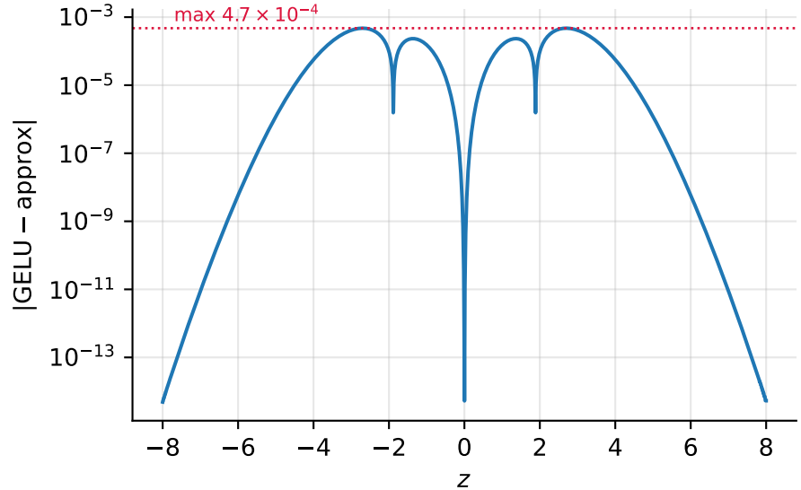
error of the tanh approximation (8.geluapprox)
