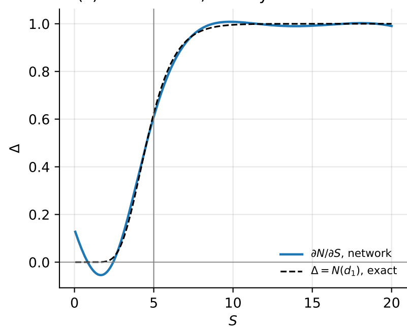
(c) the Greek \Delta , free by differentiation
