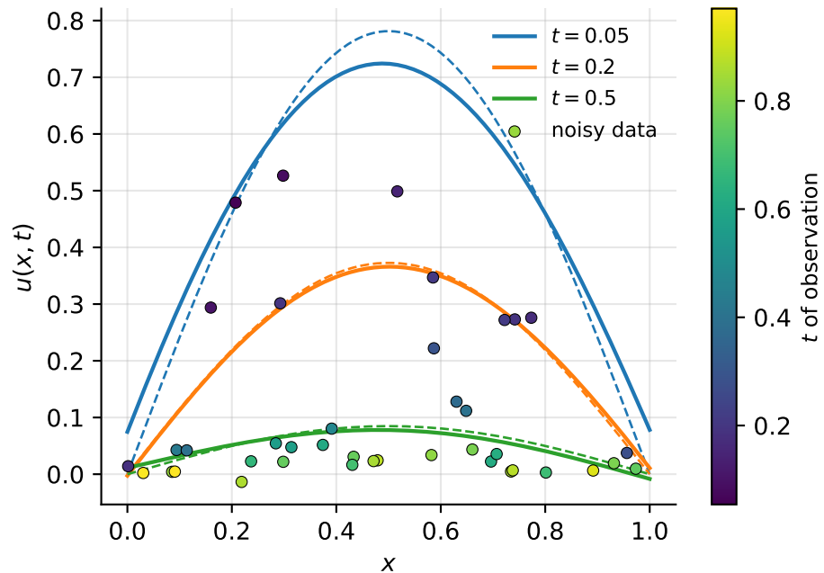
(b) solution and the 40 observations
