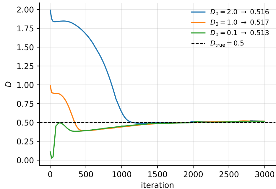
(a) the unknown coefficient is recovered
