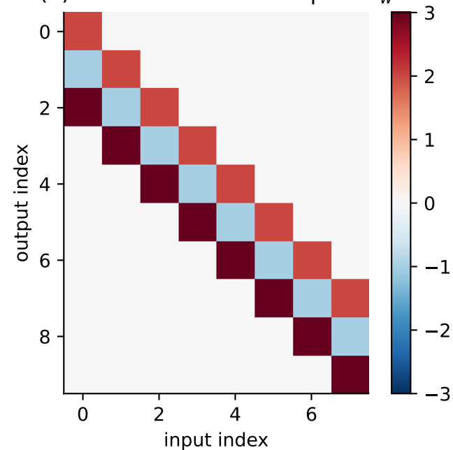
(a) 1-D convolution: Toeplitz \mathbf{T}_w
