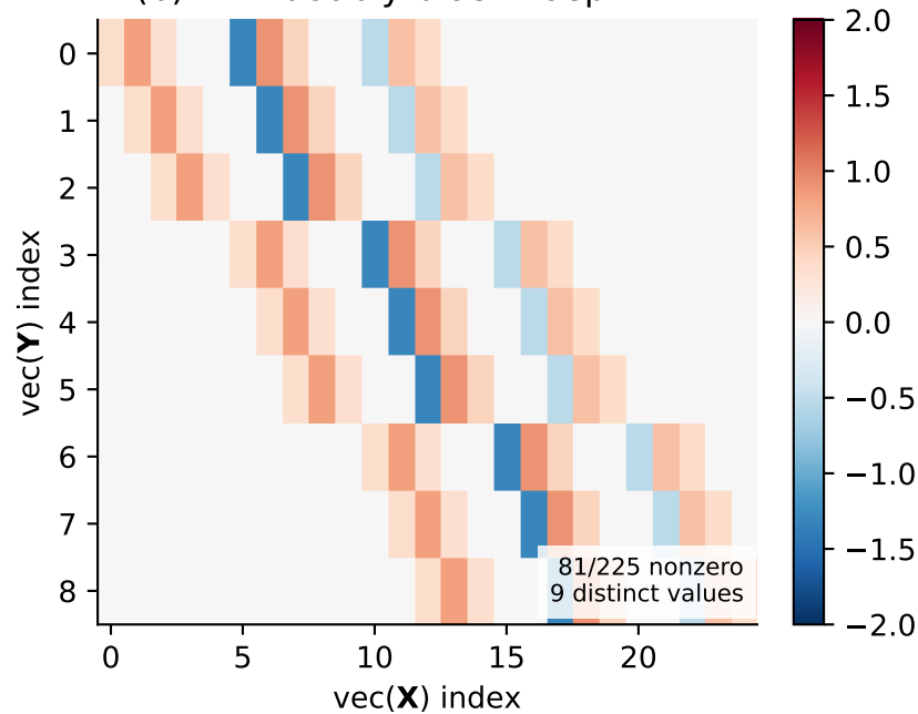
(b) 2-D: doubly block Toeplitz \mathbf{W}'
