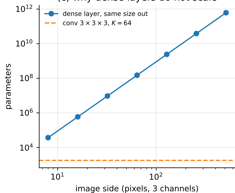
(c) why dense layers do not scale
