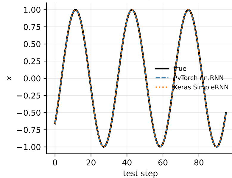
(a) one step ahead
