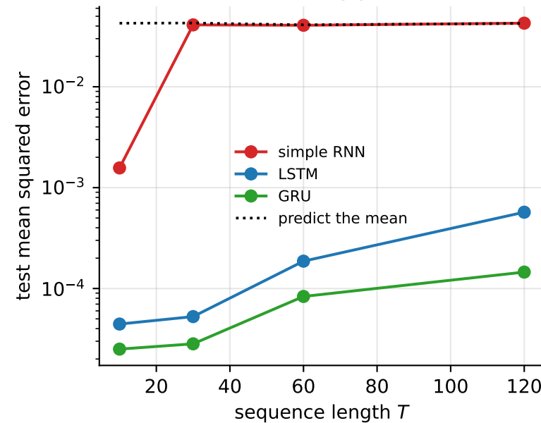
(c) the adding problem
