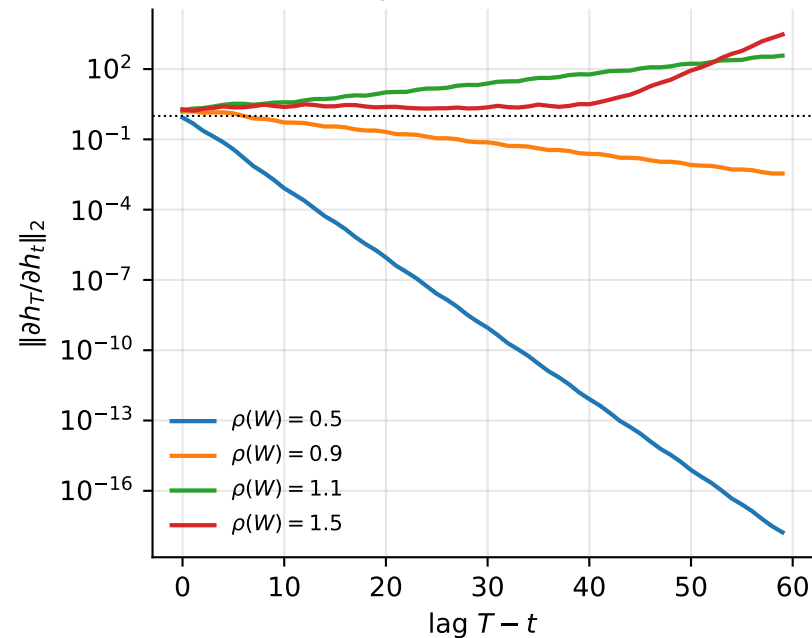
(a) the product of Jacobians
