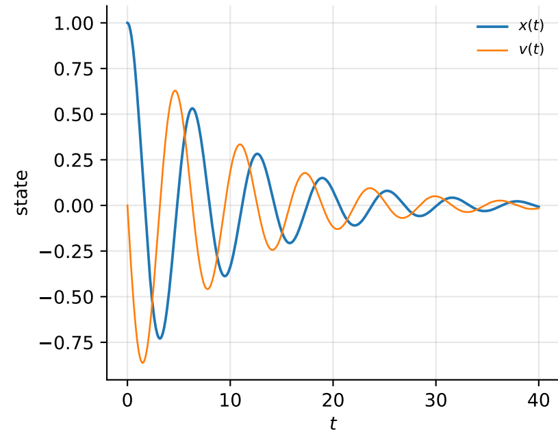
(a) \ddot{x} + \eta \dot{x} + x = 0 by RK4
