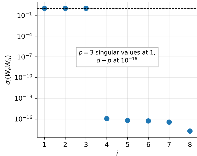
(c) W_e W_d is a rank- p projector
