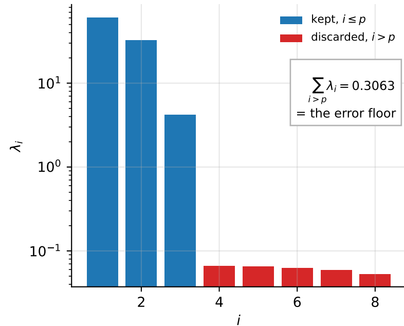
(a) spectrum of the covariance \mathbf{S}
