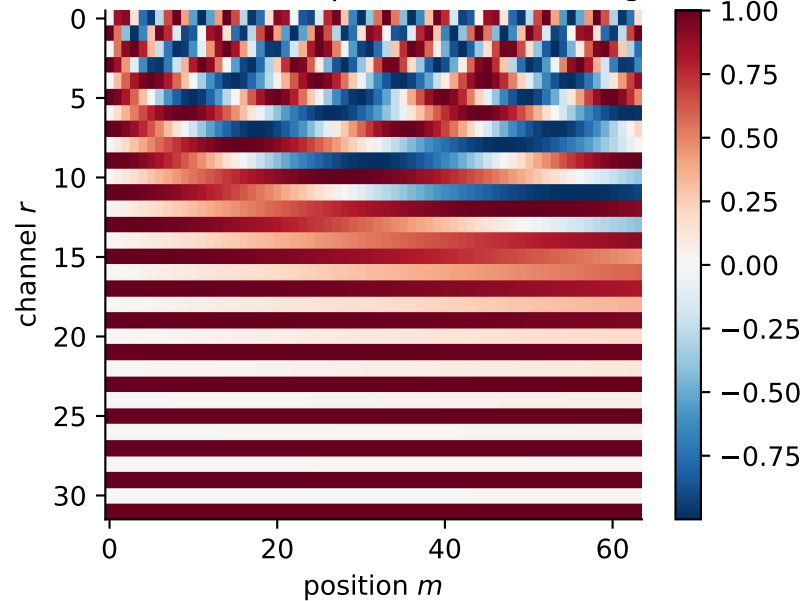
(b) sinusoidal positional encoding
