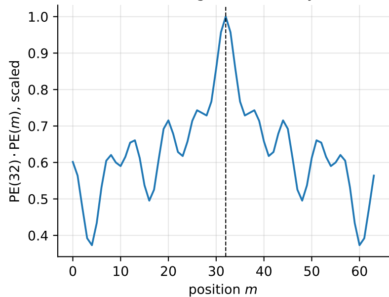
(c) the encoding is a similarity kernel
