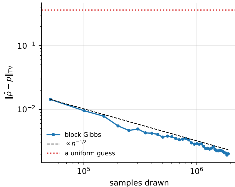
(b) Gibbs samples the model
