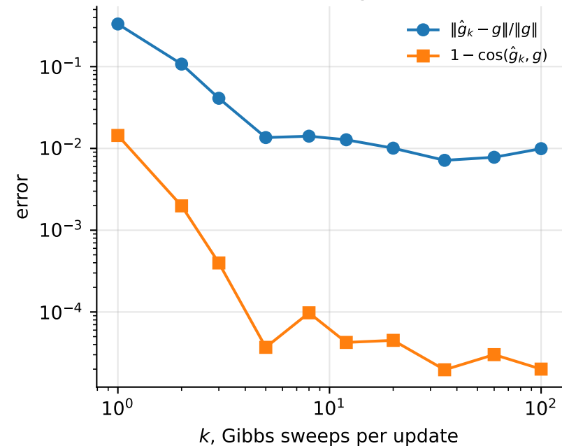
(a) contrastive divergence is biased
