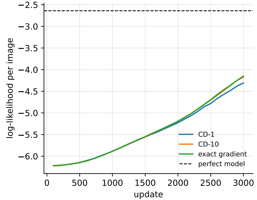
(c) what the bias costs
