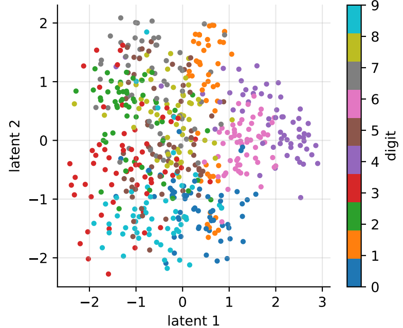
(c) the d_h = 10 latent space, projected
