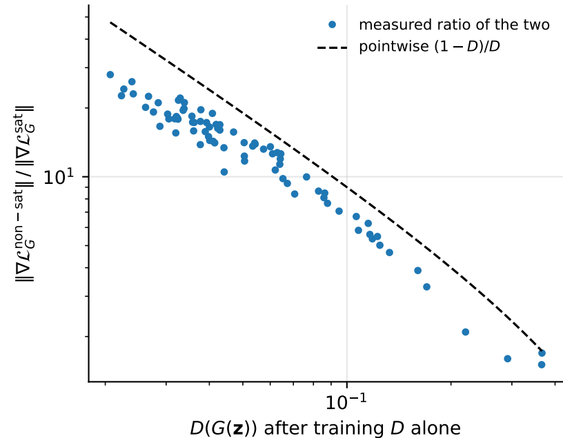
(c) gradient starvation
