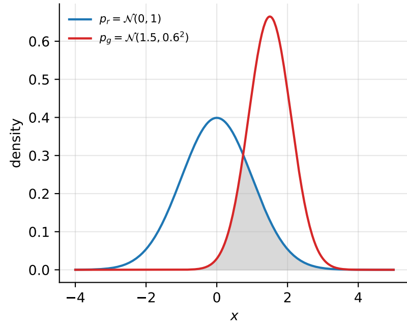
(a) the two distributions
