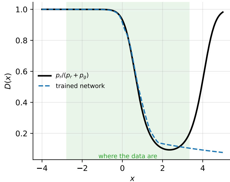
(b) the optimal discriminator
