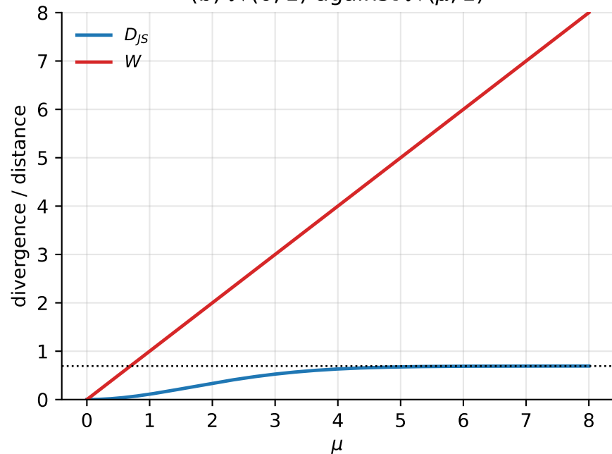
(b) \mathcal{N}(0, 1) against \mathcal{N}(\mu, 1)
