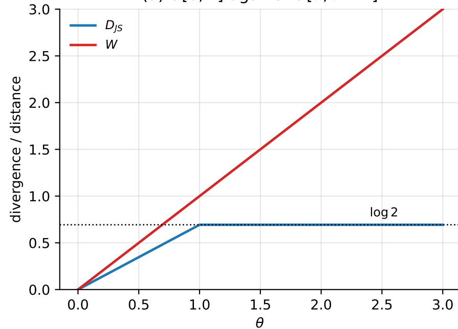
(a) U[0, 1] against U[\theta, \theta + 1]
