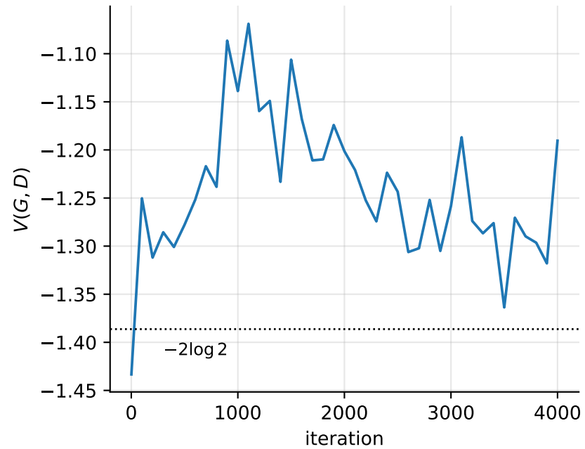
(c) the value function
