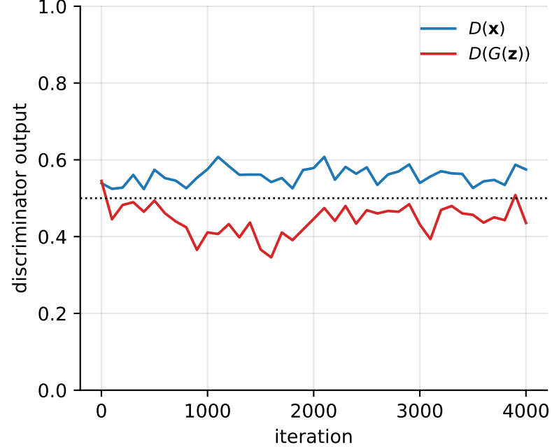
(b) the discriminator stays near 1/2
