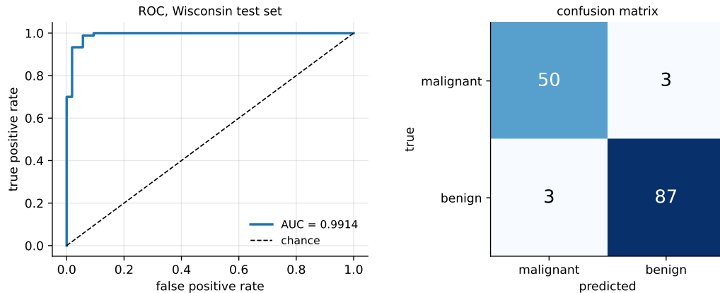
Fig. 5.6 Logistic regression on the Wisconsin test set. Left: the ROC curve, with AUC = 0.9914. Right: the confusion matrix, whose off-diagonal entries are the two kinds of error and are not equally costly.
