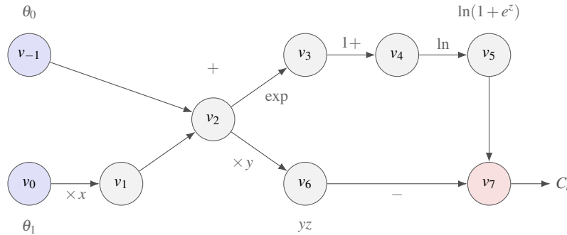
Fig. 5.4 The computational graph of the cross entropy of one observation, trace (5.35). The inputs are the two parameters; the data x and y enter as constants on the edges. The linear predictor z = v_2 fans out into the softplus branch along the top and the label branch along the bottom, and the reverse sweep of Eq. (5.38) sums the two when it reaches v_2 , producing the residual p - y .
