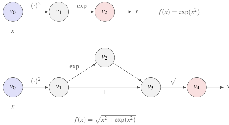
Fig. 4.9 The computational graphs of the two examples of Section 4.14.5. Top: f(x) = \exp(x^2) , trace (4.77), a chain in which every value is used once. Bottom: f(x) = \sqrt{x^2 + \exp(x^2)} , trace (4.81), where v_1 = x^2 feeds both the exponential and the sum. The two paths from v_1 to y are the two terms of the adjoint \bar{v}_1 in Eq. (4.83).
