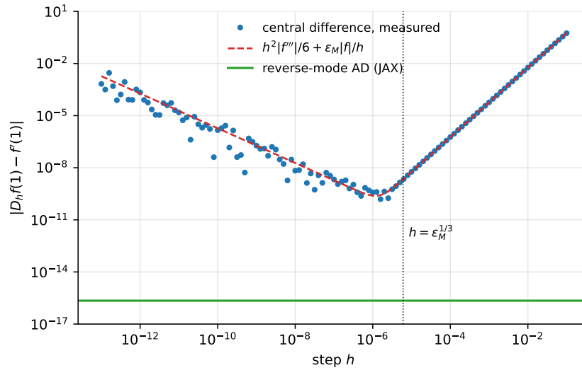
Fig. 4.10 Absolute error of the central finite difference (4.59) for f(x) = \sin(2\pi x + x^2) at x = 1 , as a function of the step h (points), together with the model (4.61) (dashed): truncation error \propto h^2 on the right, rounding error \propto 1/h on the left, and a minimum of about 10^{-10} near h \approx \varepsilon_M^{1/3} . The reverse-mode derivative computed by JAX has an error at the level of the unit roundoff, shown as the horizontal line, for any h because it involves no h .
