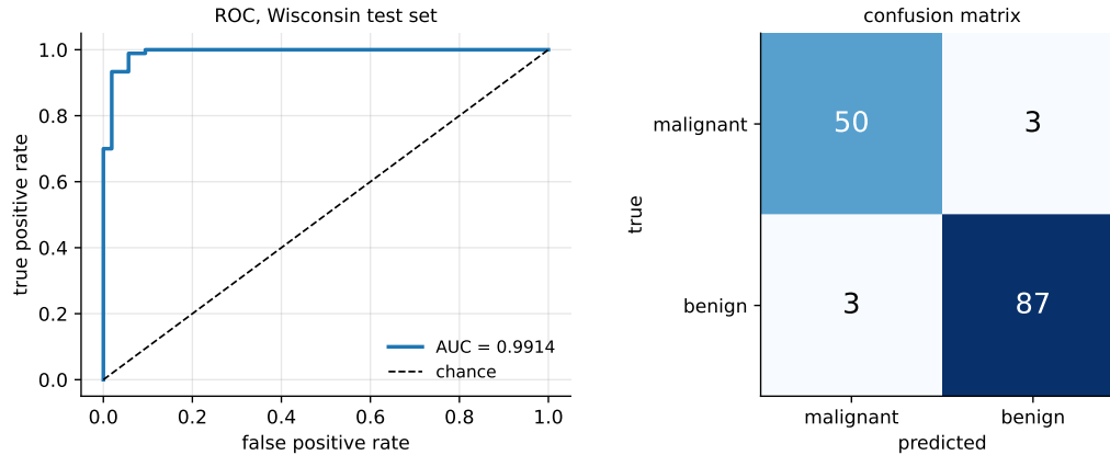
Fig. 5.9 Logistic regression on the Wisconsin test set. Left: the ROC curve, with AUC = 0.9914 . Right: the confusion matrix, whose off-diagonal entries are the two kinds of error and are not equally costly.
