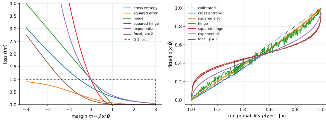
Fig. 5.8 Left: the loss functions of Table 5.2 against the margin, for a point of class \tilde{y} = +1 ; the 0–1 loss is dotted. Right: the probability \sigma(\mathbf{x}^T \hat{\boldsymbol{\theta}}) obtained by minimising each loss with a linear model on 400 points drawn from a true logistic model, plotted against the true probability. The cross entropy and the squared error follow the diagonal; the exponential loss recovers half the log-odds, so its curve is the diagonal compressed towards \frac{1}{2} ; the squared hinge and the focal loss are compressed further; the hinge loss does not estimate a probability at all.
