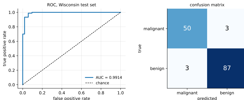
Fig. 5.4 Logistic regression on the Wisconsin test set. Left: the ROC curve, with AUC = 0.9914 . Right: the confusion matrix, whose off-diagonal entries are the two kinds of error and are not equally costly.
