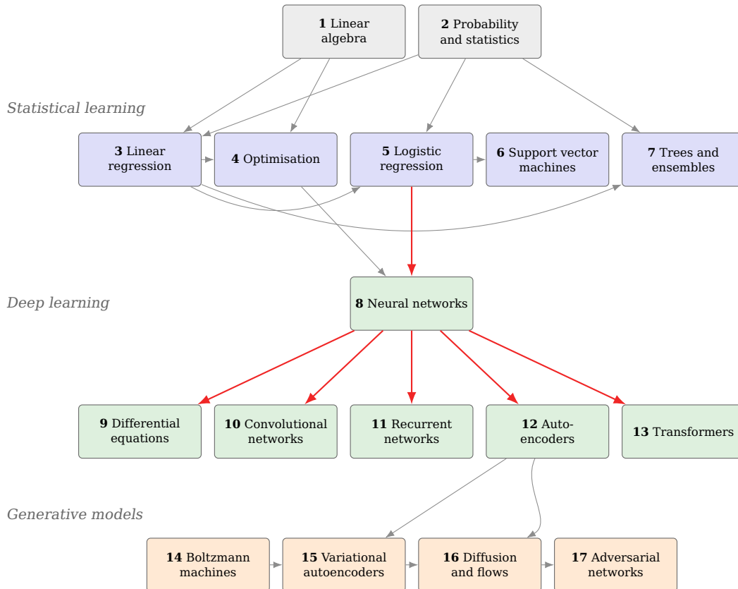
Fig. 18.1 The book as a graph. An arrow means that the later chapter uses a result of the earlier one, not merely that it comes after it. The two red paths are the ones the book is built around: logistic regression is a network with no hidden layer, so Chapter 8 begins by inserting one; and Chapters 9 to 13 all use the backpropagation of Section 8.8 unchanged – Chapters 10 to 13 by changing what structure is imposed on the weight matrix, Chapter 9 by keeping the network and changing the question it is asked. Two links are not drawn because they would cross the whole figure. The linear autoencoder of Chapter 12 rediscovers the singular value decomposition of Chapter 1 – that is Theorem 12.5 – and the Boltzmann machine of Chapter 14 is sampled by the Metropolis algorithm of Section 2.14.
