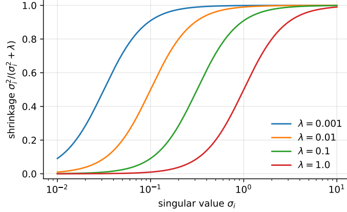
Fig. 3.1 The Ridge shrinkage factor \sigma_i^2/(\sigma_i^2 + \lambda) of Eq. (3.32) against the singular value, for four penalties. The transition is centred on \sigma_i = \sqrt{\lambda} .
