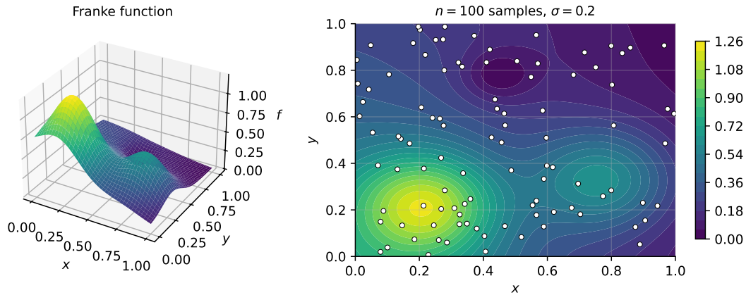
Fig. 3.3 The Franke function (3.75) on the unit square (left) and a contour view with the n = 100 noisy samples used in this section marked (right). Two peaks, a saddle and a depression make it too rich for a low-order polynomial and well within reach of a moderate one.
