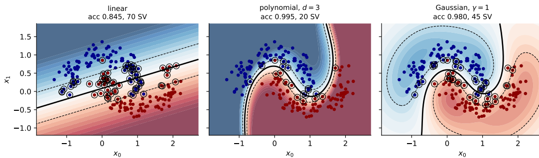
Fig. 6.3 Decision functions for three kernels on the moons data, all fitted with the solver of Section 6.10. Solid contour: the boundary; dashed: the \pm 1 margins; circles: support vectors. Colour shows the value of Eq. (6.33) before the sign is taken.
