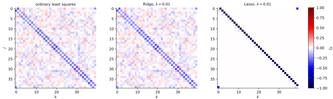
Fig. 3.6 The coupling matrices J_{jk} recovered from 400 configurations of the L = 40 Ising chain. The truth is a single off-diagonal band. OLS and Ridge spread the interaction over the whole matrix and split each coupling symmetrically between (j, k) and (k, j) ; the Lasso finds the band and puts each coupling entirely on one side of the pair. Both behaviours are forced, by Proposition 3.12.
