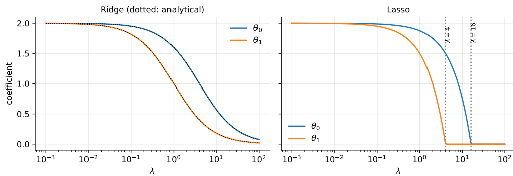
Fig. 3.2 Coefficient paths for the toy problem (3.54). The Ridge coefficients (left) follow the analytical result (3.57), shown dotted, and approach zero only asymptotically. The Lasso coefficients (right) reach zero at the finite thresholds \lambda = 4 and \lambda = 16 predicted by Eq. (3.47).
