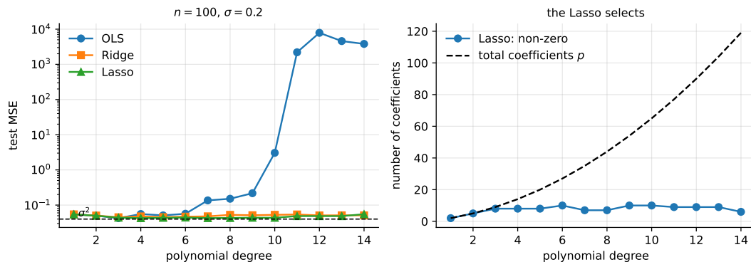
Fig. 3.4 Test error against polynomial degree for the three estimators on the Franke data (left, logarithmic), with the noise floor \sigma^2 = 0.04 marked; and the number of coefficients the Lasso retains against the total number available (right).
