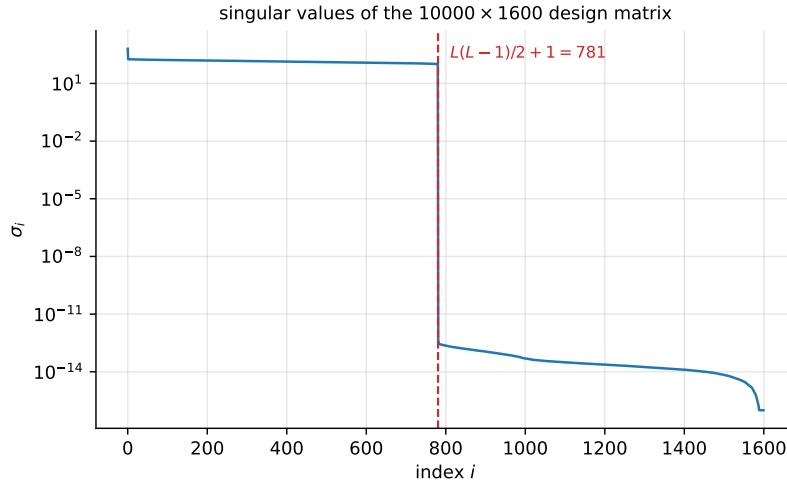
Fig. 3.5 Singular values of the 10000 \times 1600 Ising design matrix (3.78) for L = 40 . The spectrum collapses precisely at the index L(L-1)/2 + 1 = 781 predicted by Proposition 3.11: the rank deficiency is a property of the features, not of the sample.
