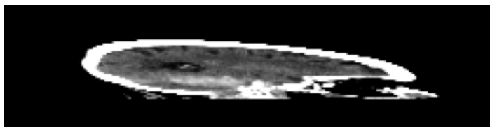
Sagittal Image
