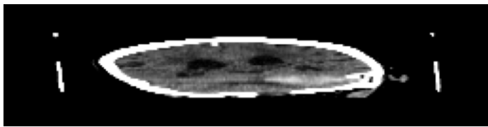
Coronal Image
