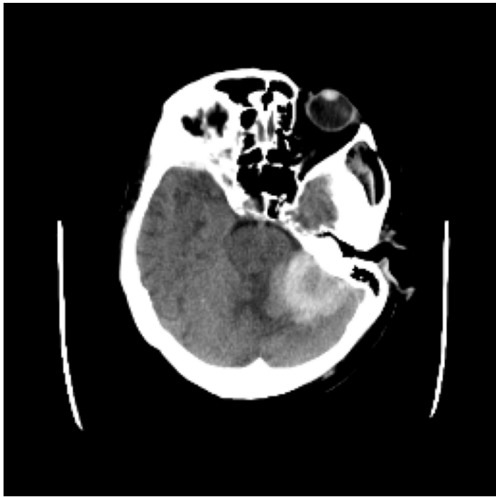
Axial Image
