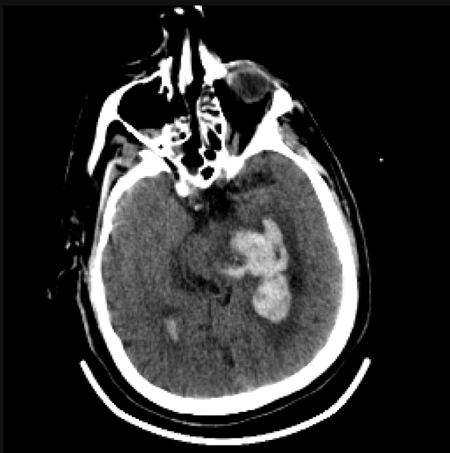
Axial (+3) Image
