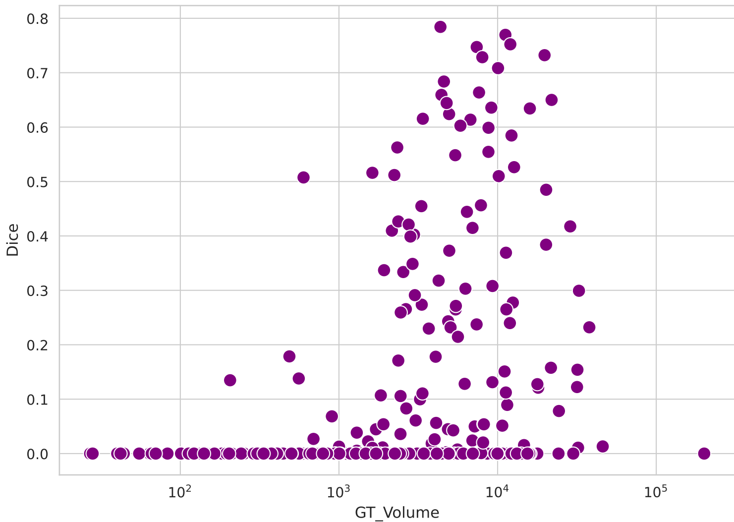
Dice vs Ground Truth Volume
