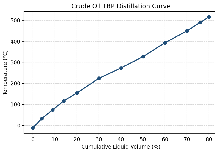
Figure 4: True boiling point (TBP) distillation curve of the crude feed.
