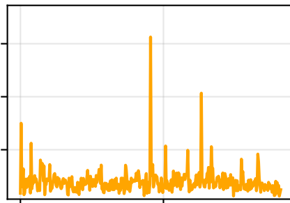
XGB
