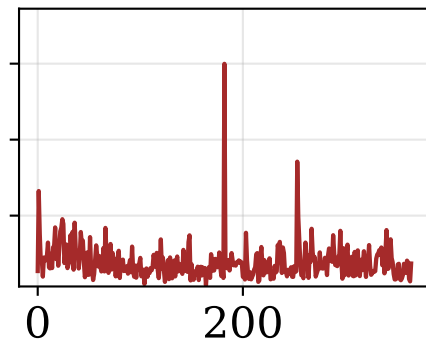
TFT
