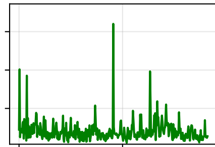
DNN
