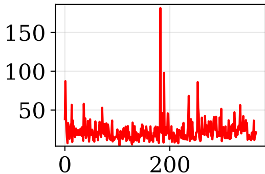
LEAR
