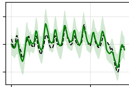
TFT
