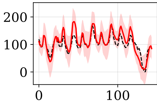
LEAR
