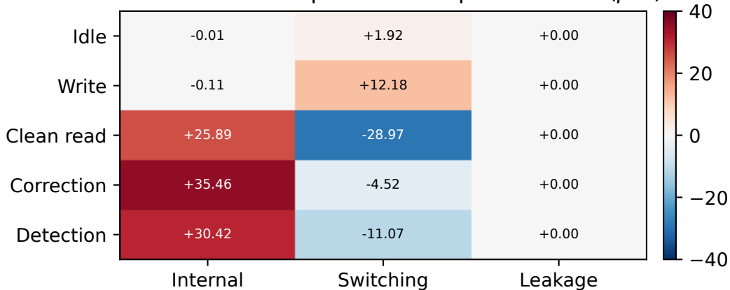
Candidate heatmap: mean component delta ( \mu\text{W} )
