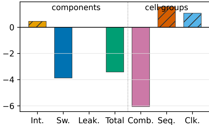
(a) 10 ns power accounting
