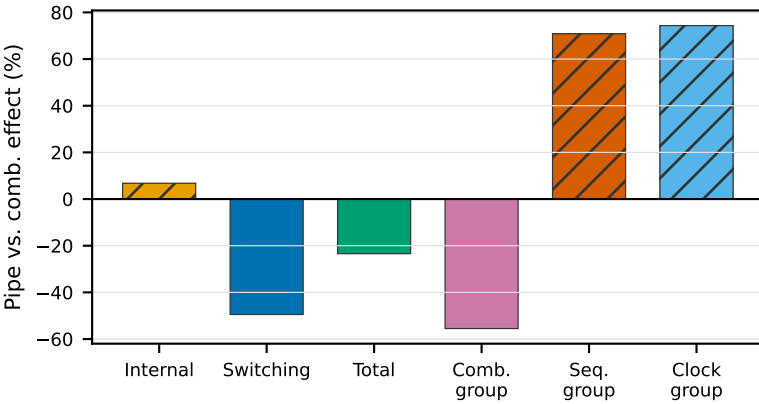
(a) 10 ns power decomposition
