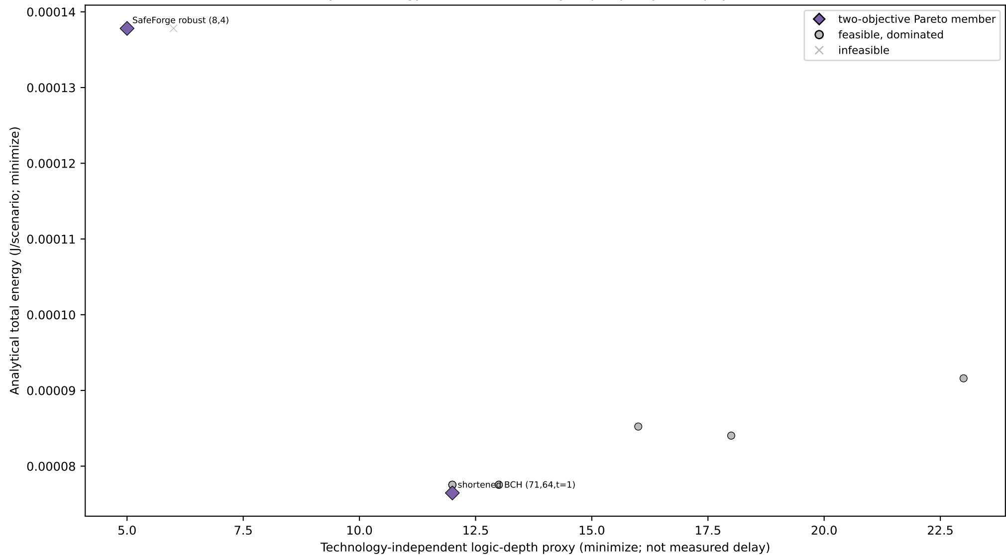
Energy-complexity Pareto frontier Analytical energy and structural-only depth proxy—not physical PPA
