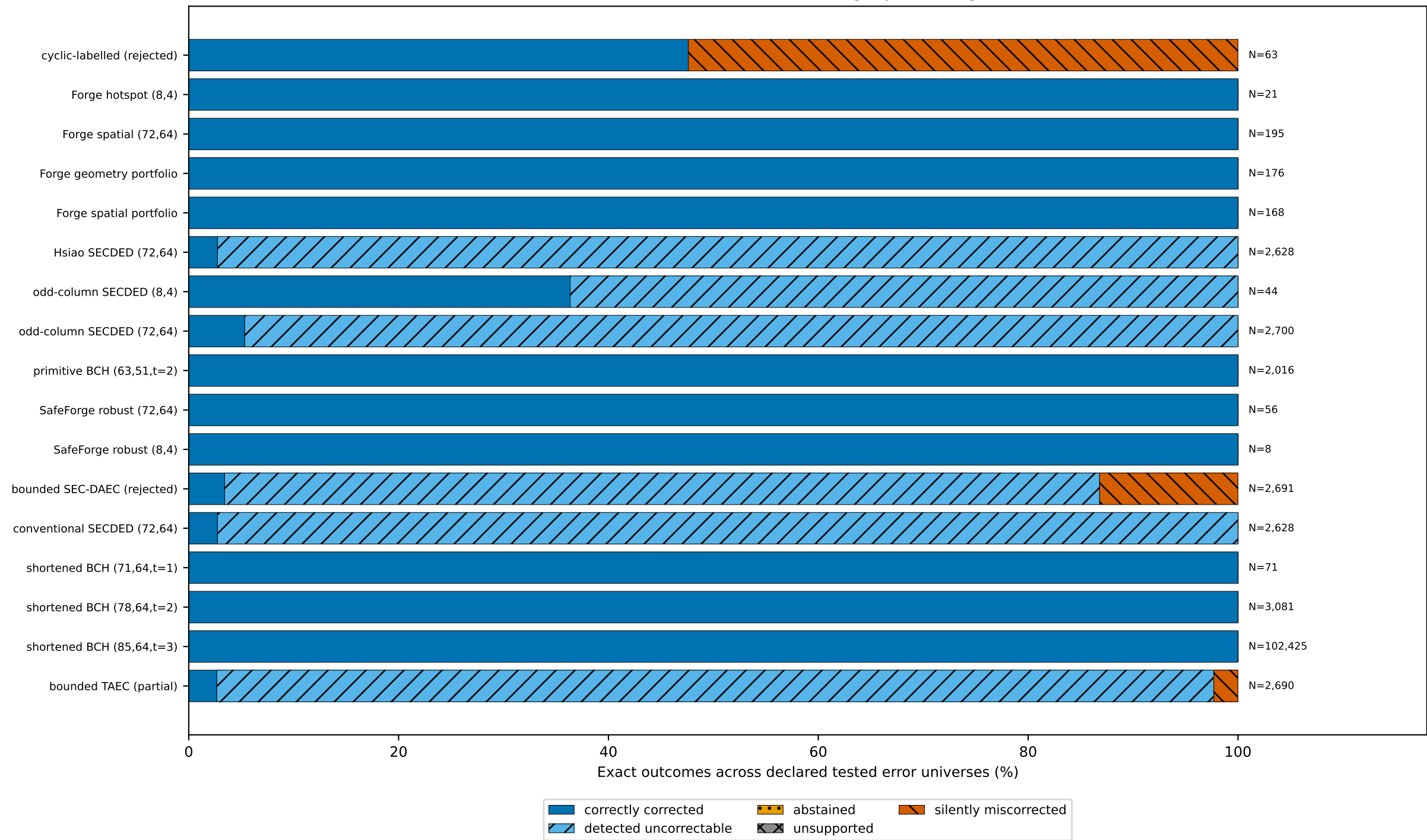
Exact verification outcomes, including rejected negative results
