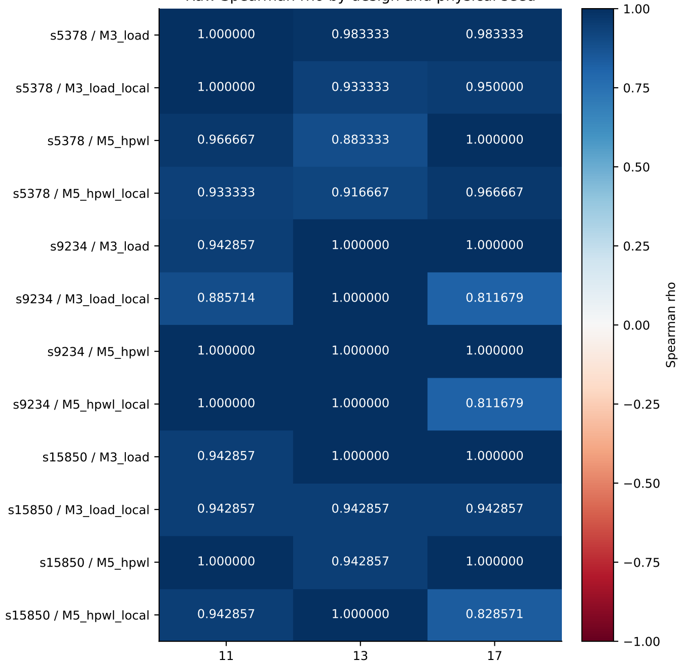
Raw Spearman rho by design and physical seed
