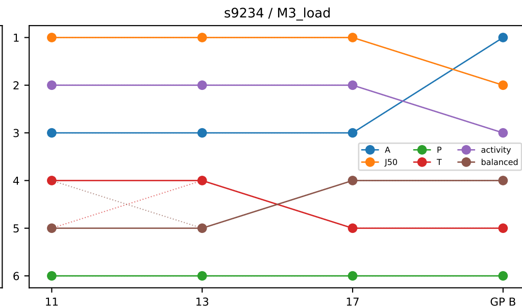
Architecture ranking stability: solid target, dotted predictor Average ranks for ties; rank 1 is the smallest score
