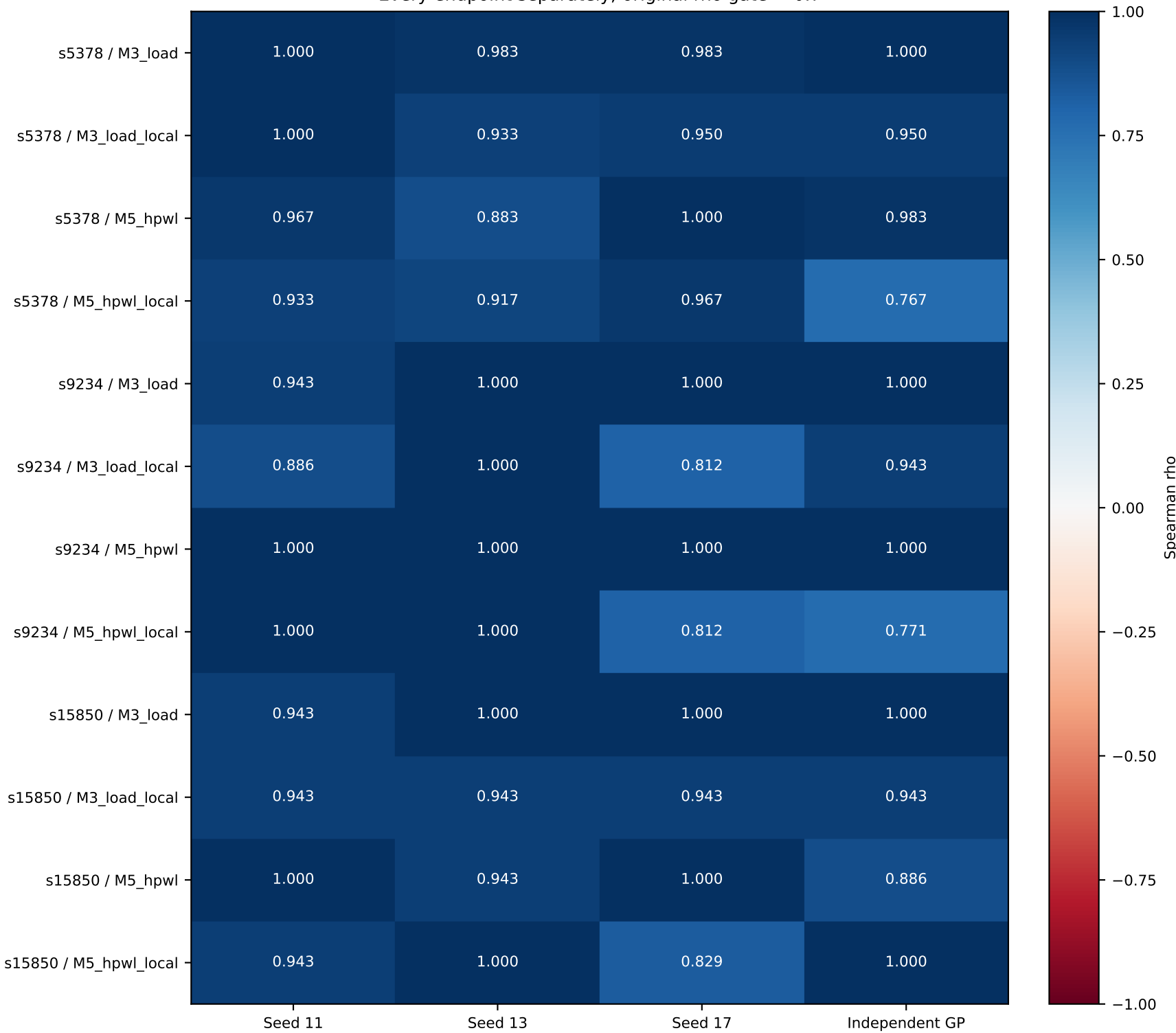
Every endpoint separately; original rho gate = 0.7
