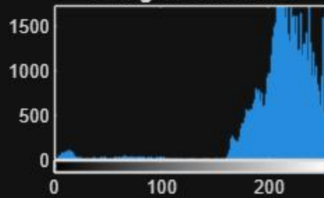
Histogram Bar Plot
