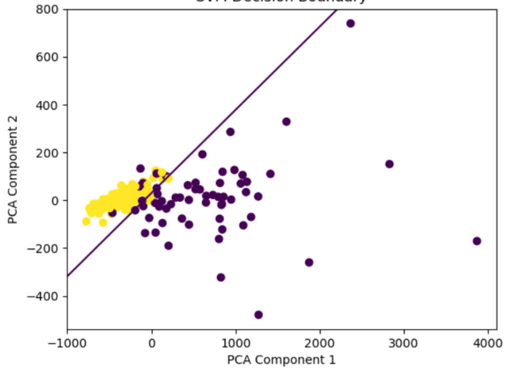
SVM Decision Boundary
