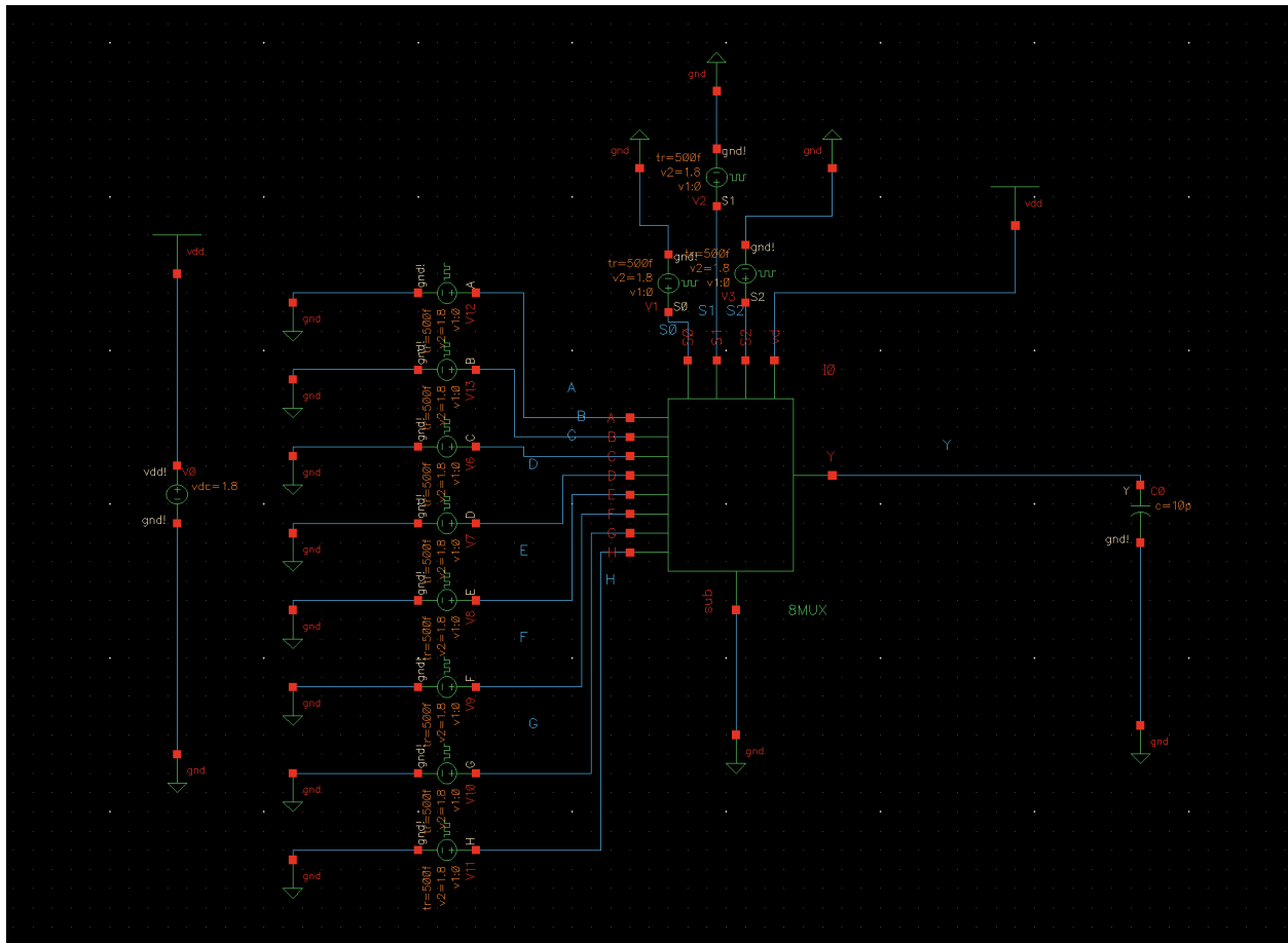
Schematic used to simulate 8:1 MUX
