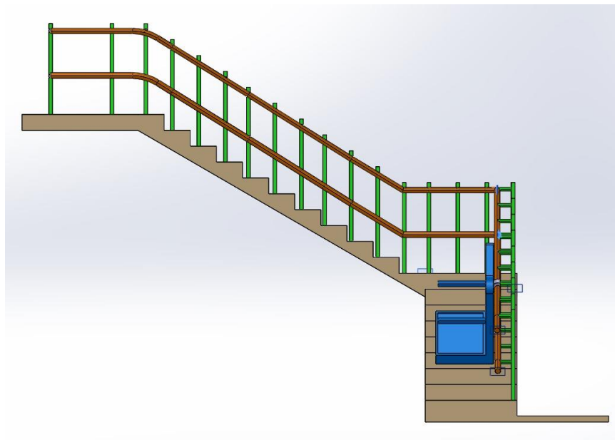
FIGURE 2: FRONT VIEW
