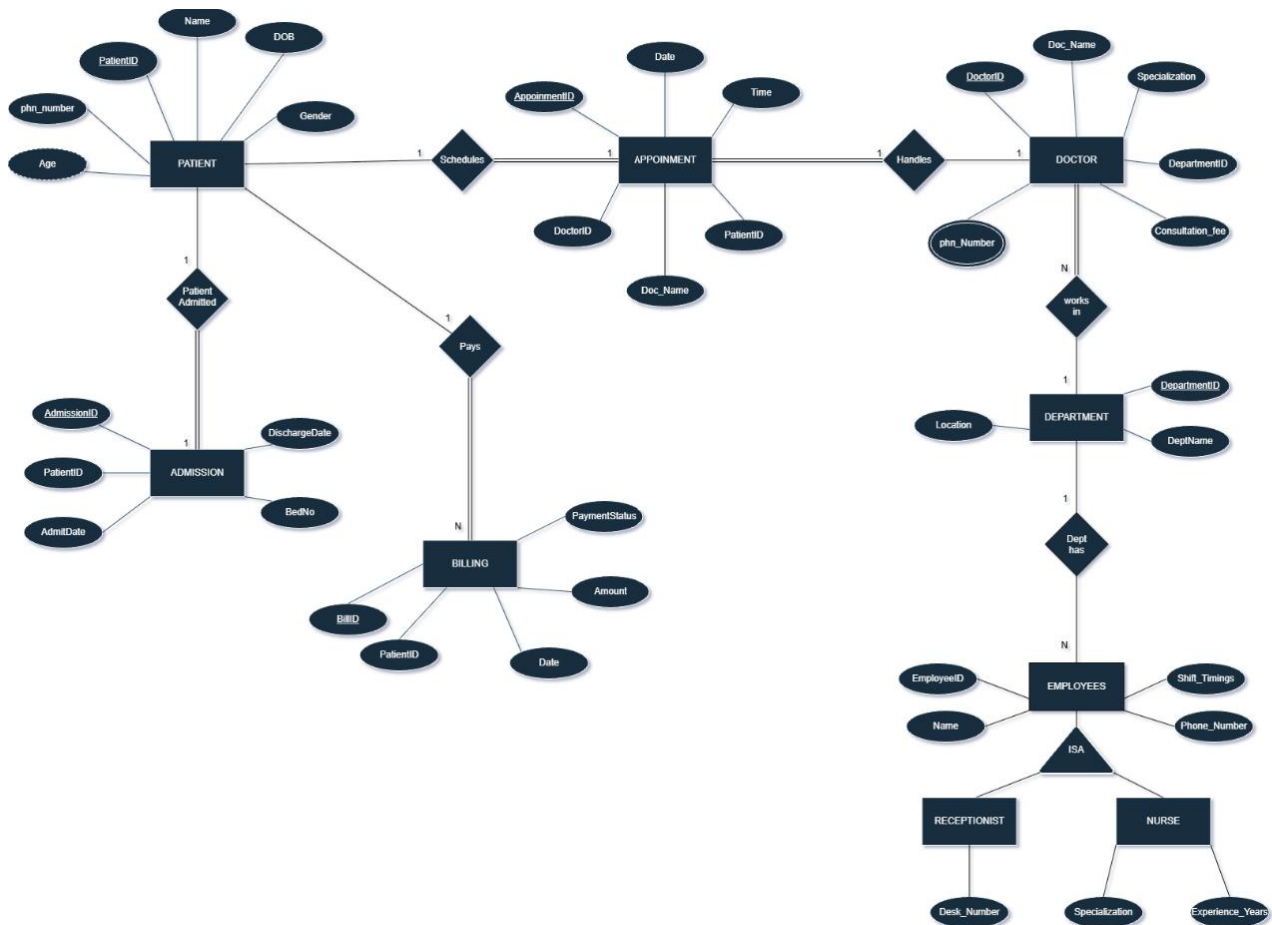
Figure 1: ER Diagram of Hospital Management System
