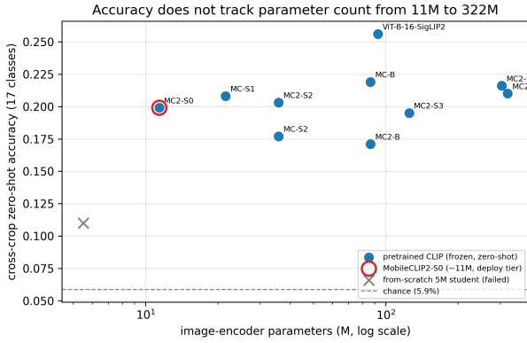
Figure 1: Zero-shot accuracy against image-encoder size. Cross-crop accuracy for frozen pretrained encoders spanning a 28-fold parameter range, with a from-scratch small student for contrast. The pretrained models cluster together regardless of size; the from-scratch student sits near chance.
