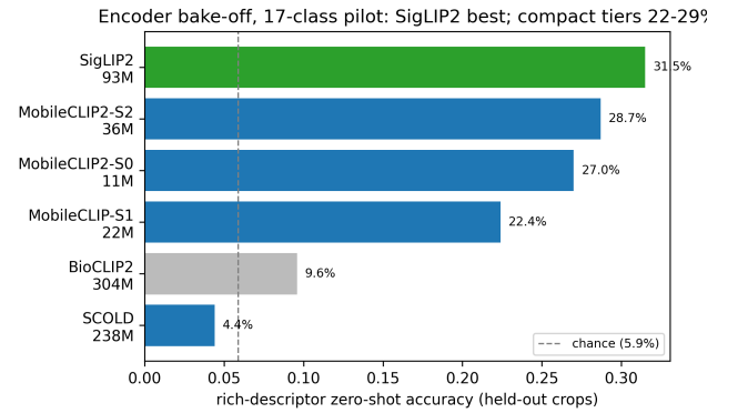
Figure 3: Encoder bake-off on the pilot held-out set. Rich-descriptor zero-shot accuracy for each candidate backbone against its image-encoder parameter count. Under this descriptor protocol the domain foundation models transfer far less well than the general-purpose compact encoders: BioCLIP2 reaches 9.6% (1.6 \times chance) against 27.0% for the 11.4 M MobileCLIP2-S0, and the SCOLD point is a best-effort load we rest no claim on (Section 4.2).
