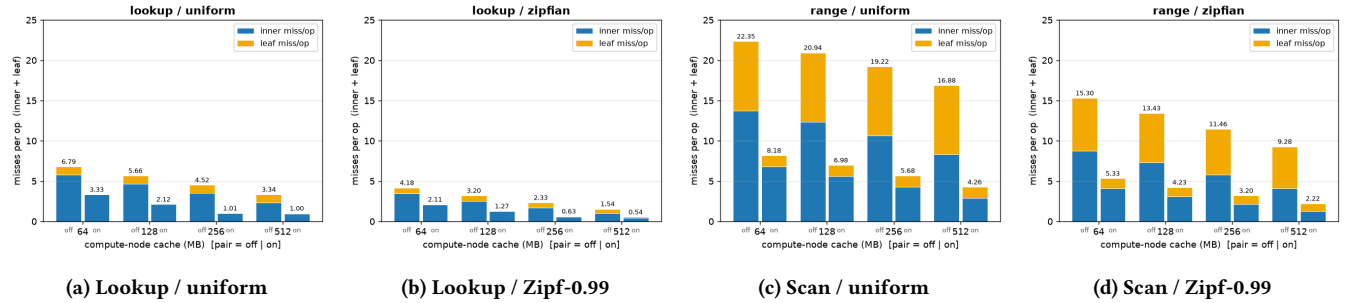
Figure 6: Misses per operation split into inner (blue) vs. leaf (amber); each bar-pair is off | on per cache. Offloaded lookups drive the leaf band to \approx 0 (the leaf is served inside the RPC); scans retain an entry-leaf component.
