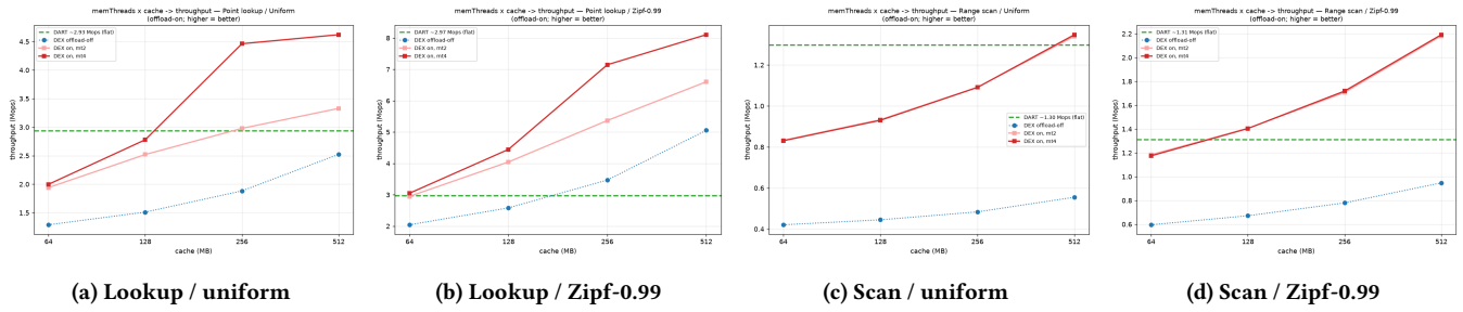
Figure 11: Joint memThreadCount \times cache effect on DEX offload-on throughput, with DEX offload-off and DART's flat baseline for reference. More threads lift the whole curve while the memory node is the bottleneck; the lift shrinks once cache makes the compute/network side the limit.
