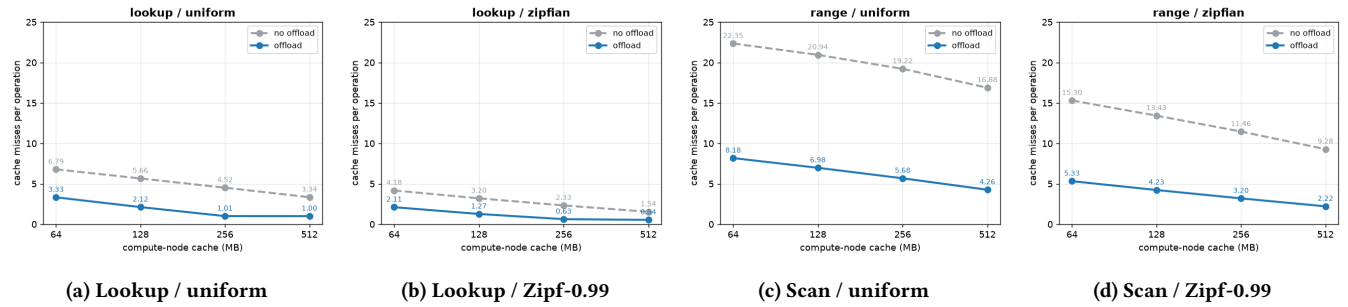
Figure 5: Total misses per operation vs. cache (fixed denominator; 2 cores; shared 0–25 scale). Offloading (blue) is \leq no-offloading (grey) in every panel; both fall with cache and skew.
