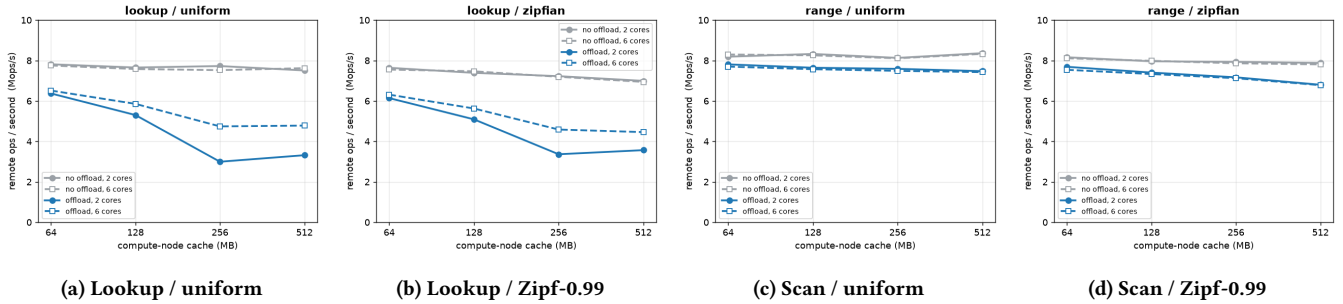
Figure 9: Aggregate remote-traffic rate (throughput \times ops/op). Here 2 vs. 6 cores diverge: more service threads let throughput climb, delivering more remote ops/s to the memory node.
