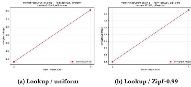
Figure 10: Throughput vs. memThreadCount (offload-on, largest cache). Throughput rises while the memory node is the bottleneck, then flattens past ~4 threads.
