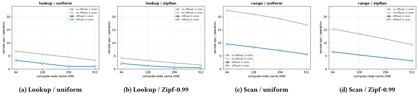
Figure 7: Remote traffic per operation , four series (offload off/on \times 2/6 cores). The 2- and 6-core markers overlap: per-op traffic is compute-side, set by cache misses, not by memory-node threads. Offloading is the lever.
