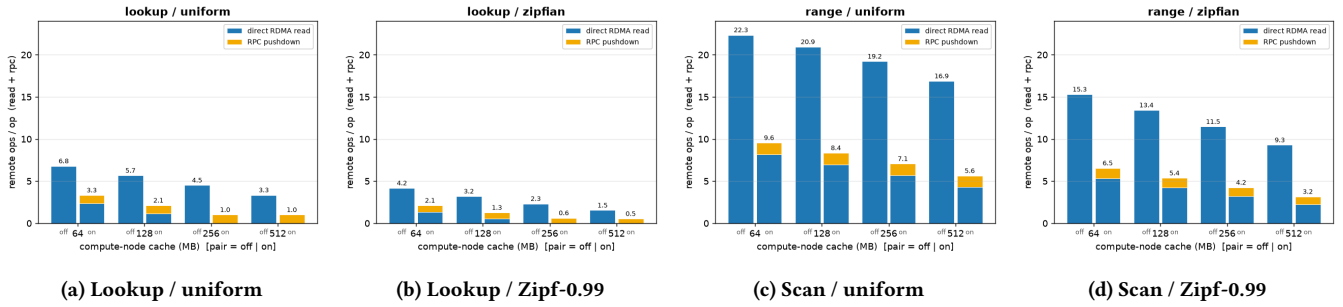
Figure 8: Composition of remote traffic per op: direct RDMA reads (blue) vs. RPC pushdowns (amber), off/on per cache (2 cores). Offloading converts reads into a much smaller number of RPCs.
