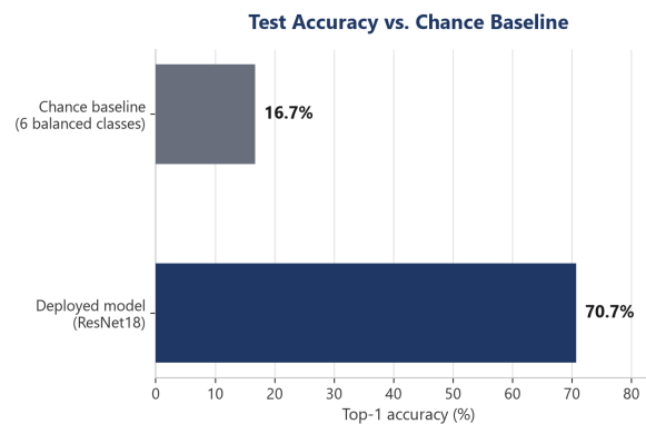
Accuracy Chart
